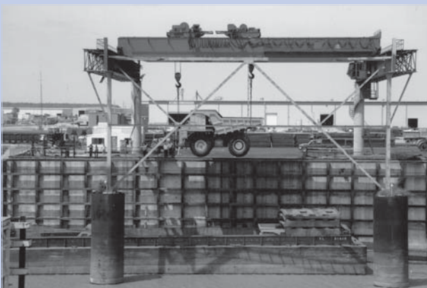
Dry cargo dock bridge crane at Tulsa Port of Catoosa lowers 205-ton quarry truck—built in Tulsa—onto jumbo hopper barge for shipping to Philippines.
