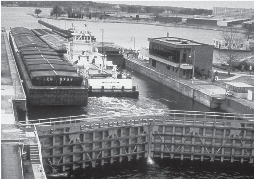
Aerial view of Lock and Dam 15, Mississippi River, Rock Island, Illinois.
