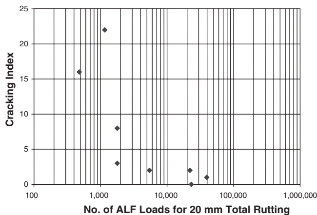
FIGURE B17 Comparison of HMA rutting to UTW cracking.
