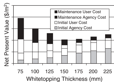
FIGURE 4 Example of LCC comparison of various whitetopping thickness strategies.
