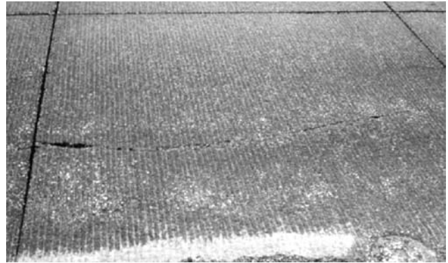
FIGURE 33 Typical midpanel crack on a UTW.
