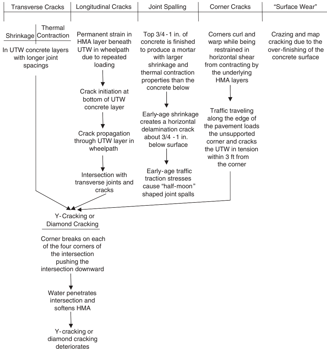
FIGURE 28 Fault tree indicating distress development for UTW (2).
