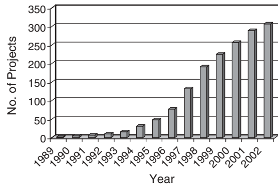
FIGURE 3 UTW construction in the United States.
