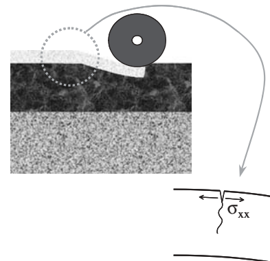
FIGURE B19 Corner cracking mechanism in a UTW slab.
