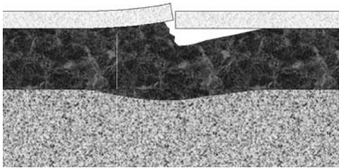
FIGURE B23 Transverse joint faulting mechanism in ALF UTW slabs.
