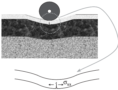
FIGURE B20 Mid-slab cracking mechanism in a UTW slab.
