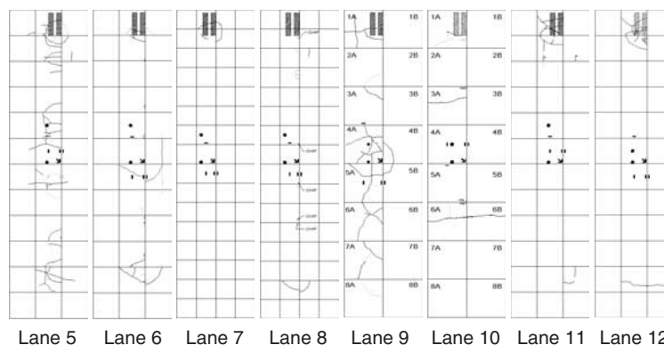
FIGURE B9 Schematic of UTW lanes at the FHWA ALF.
