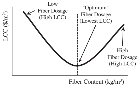
FIGURE 6 Optimizing fiber content using LCC.
