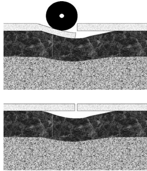
FIGURE B18 Permanent deformation of an HMA base.
