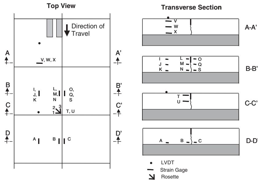
FIGURE B10 Typical schematic of sensor locations.
