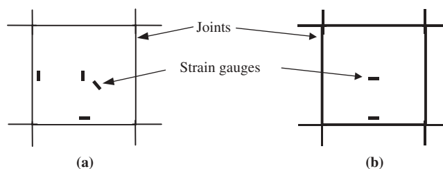
FIGURE B6 Plan view of the location of embedment strain gauges: (a) typical pattern; (b) pattern for slabs with four free edges.
