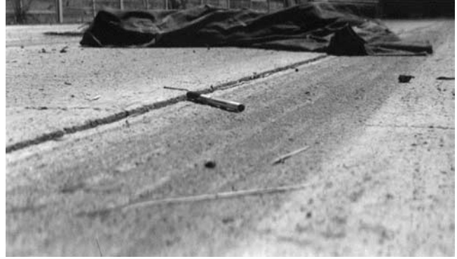
FIGURE B14 Typical UTW longitudinal faulting at the FHWA ALF.
