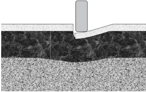
FIGURE B22 Longitudinal joint faulting mechanism in ALF UTW slabs.
