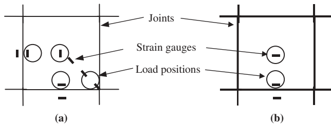
FIGURE B8 Pattern for surface strain gauges and truck loading: (a) typical pattern; (b) pattern for slabs with four free edges.
