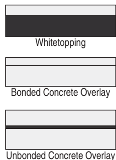
FIGURE 1 Concrete overlay types.
