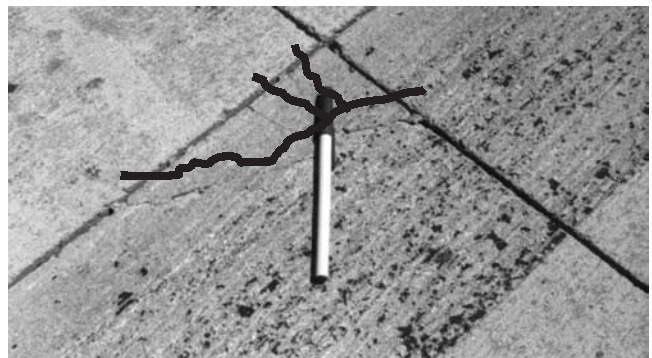
FIGURE B15 Typical UTW deflection spalling at the FHWA ALF.
