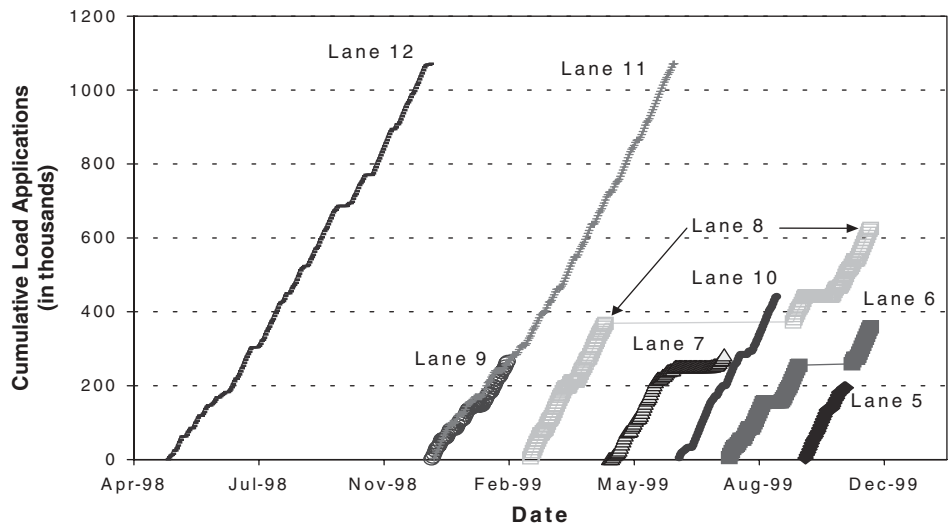
FIGURE B11 Loading history of the ALF UTW pavements.
