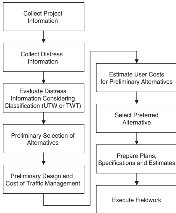
FIGURE 29 Flowchart for evaluating recommended rehabilitation activity (57).
