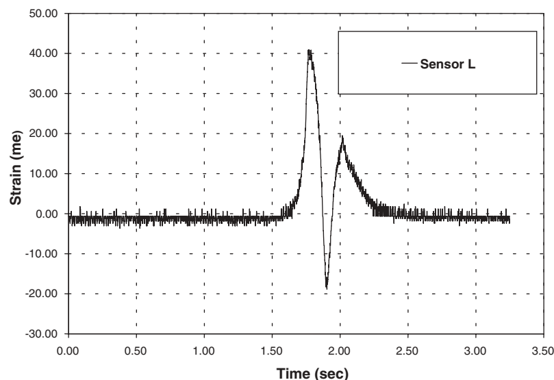
FIGURE B21 Measured strain response of a top mid-slab longitudinal gauge.
