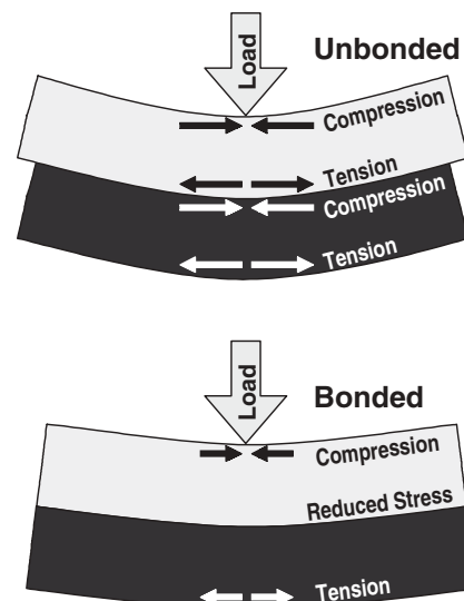
FIGURE 2 Effect of composite action on UTW and TWT behavior under flexural loading.
