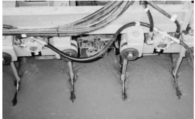
FIGURE 16 DBI submerging dowels.
