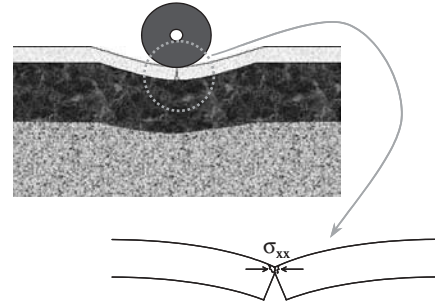
FIGURE B24 Joint spalling mechanism in ALF.
