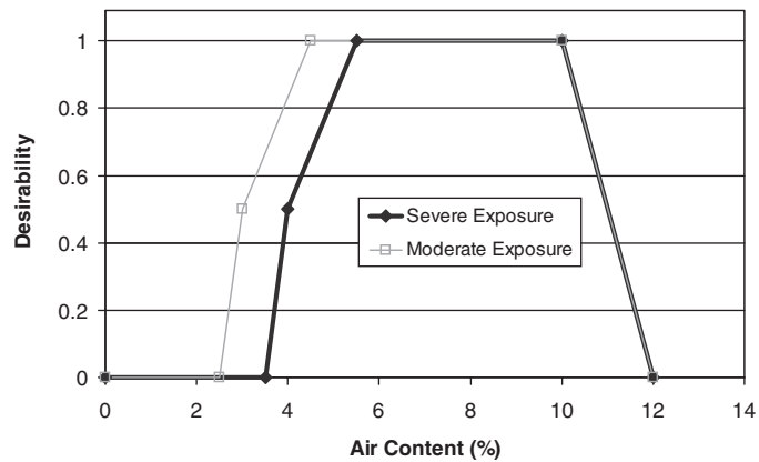
Figure S1.10. Desirability functions for air content.
