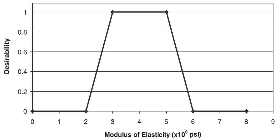
Figure S1.24. Desirability function for modulus of elasticity at 7 days.
