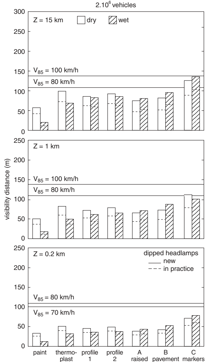
Figure 2-2. Visibility distance 22 months after application of the markings (27).
