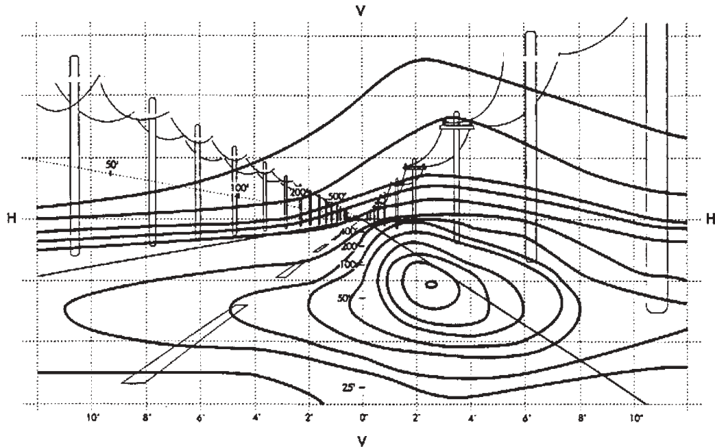
Figure 2-3. Isocandela diagram of a typical U.S. low-beam pattern superimposed on a road scene (18).
