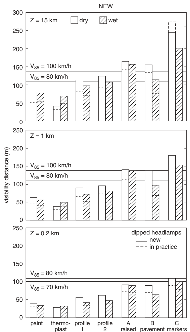
Figure 2-1. Predicted visibility distances immediately after application for all markings on a dry and wet pavement ( Z = atmospheric visibility distance) (27).
