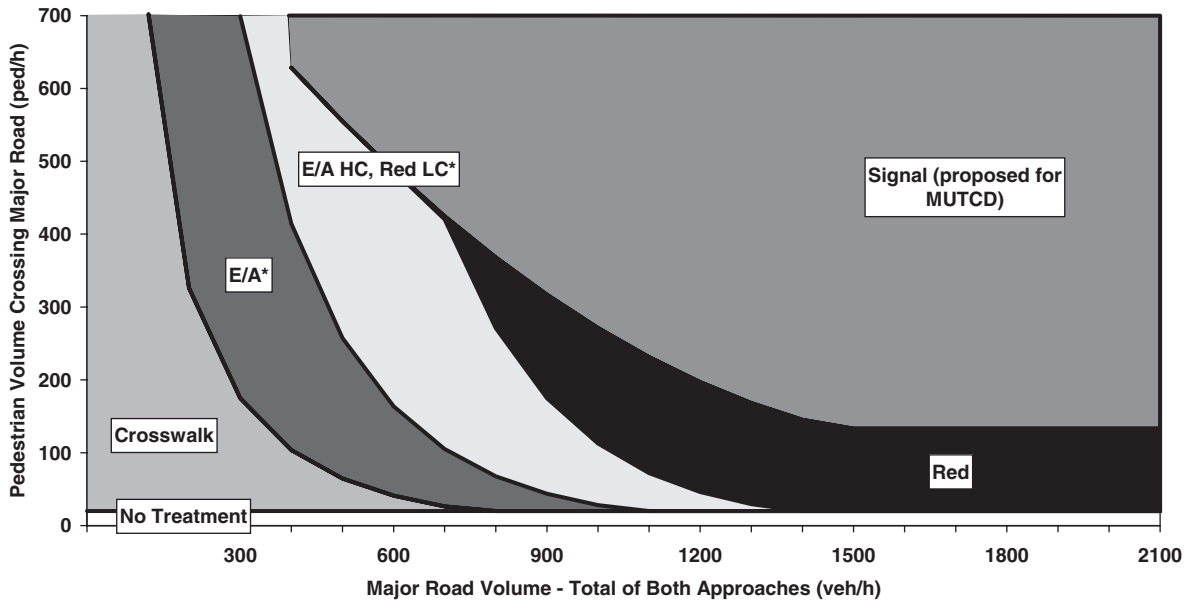
Figure A-8. Guidelines Plot, 56 ft (17 m) Pavement, ≤35 mph (55 km/h), 3.5 ft/s (1.1 m/s) Walking Speed.
