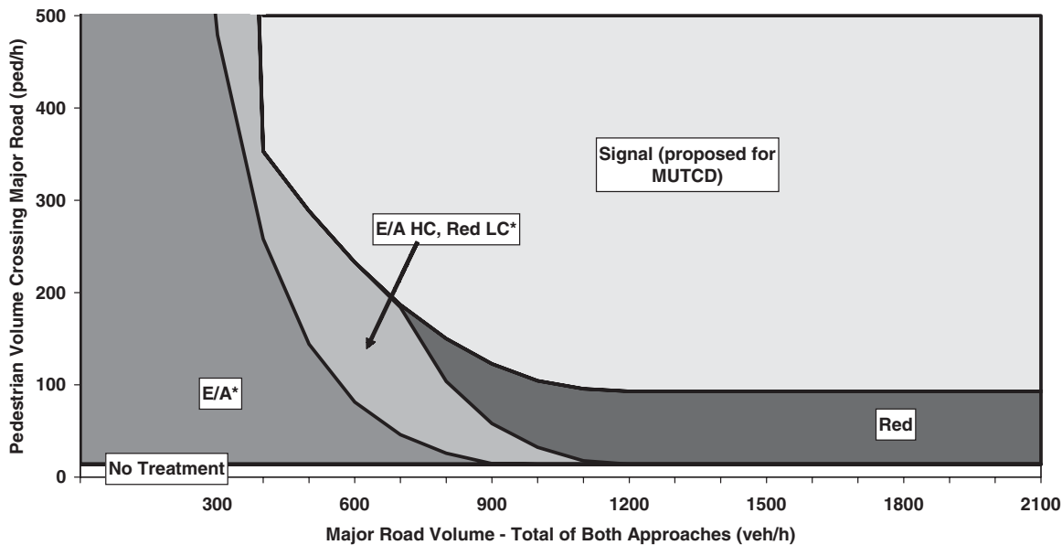
Figure A-11. Guidelines Plot, 50 ft (17 m) Pavement, >35 mph (55 km/h), 3.5 ft/s (1.1 m/s) Walking Speed.
