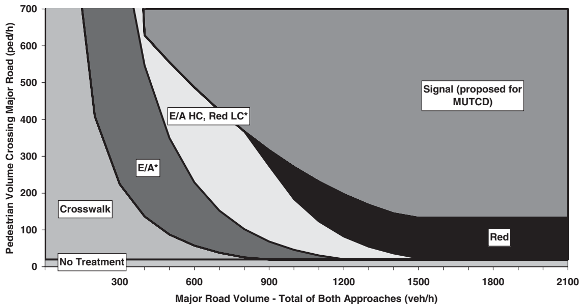
Figure A-10. Guidelines Plot, 50 ft (17 m) Pavement, ≤35 mph (55 km/h), 3.5 ft/s (1.1 m/s) Walking Speed.
