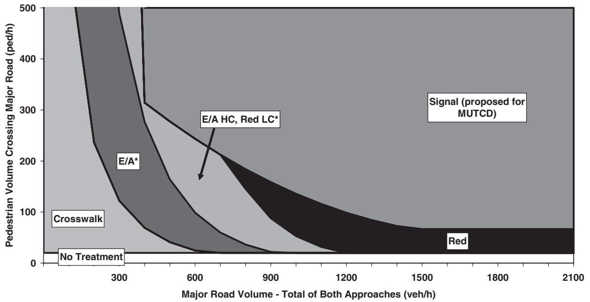
Figure A-9. Guidelines Plot, 56 ft (17 m) Pavement, ≤35 mph (55 km/h), 3.0 ft/s (0.9 m/s) Walking Speed.
