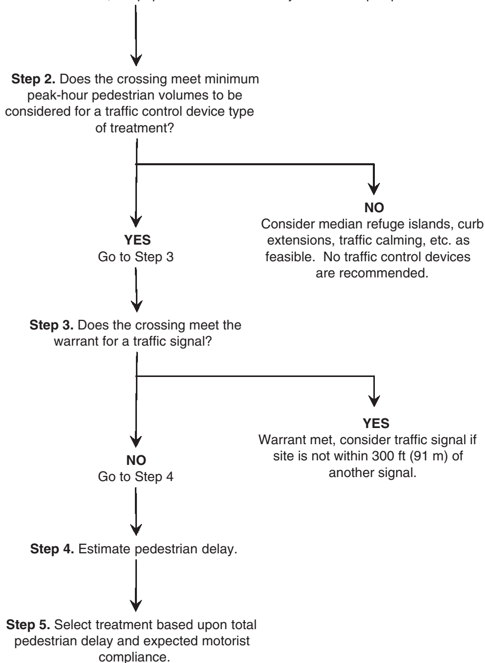
Figure A-1. Flowchart for Guidelines for Pedestrian Crossing Treatments.
