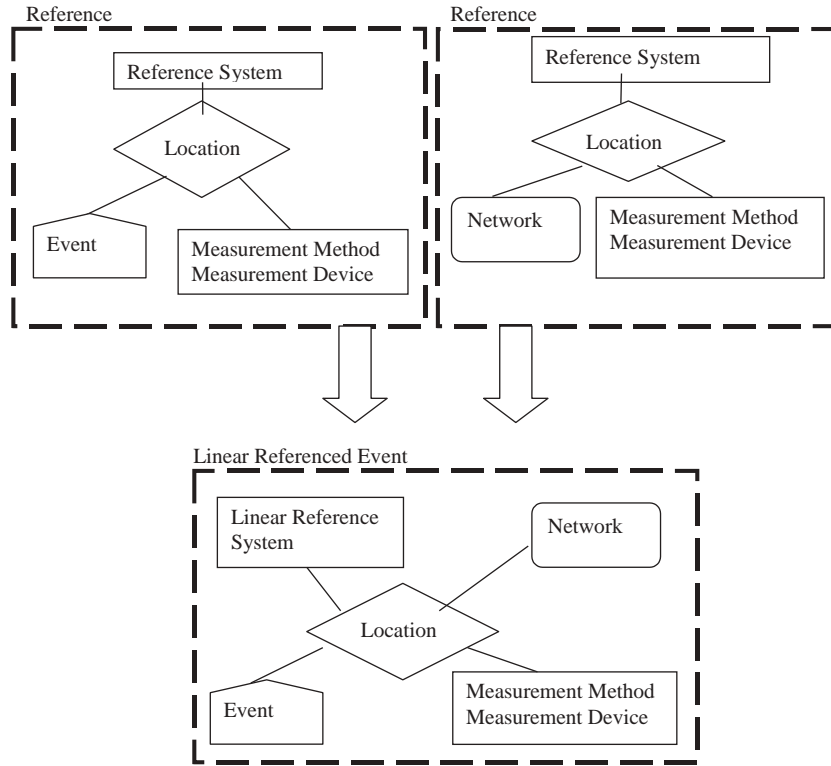
Figure 2-12. Data error model—combination of event and network.
