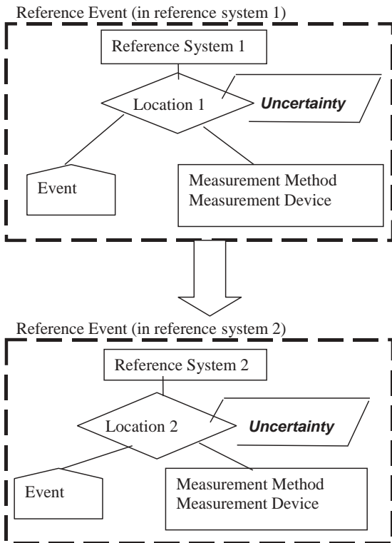
Figure 2-13. Data error model—transformation between referencing systems.
