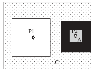
Figure 2-15. Two point locations along with their confidence intervals.
