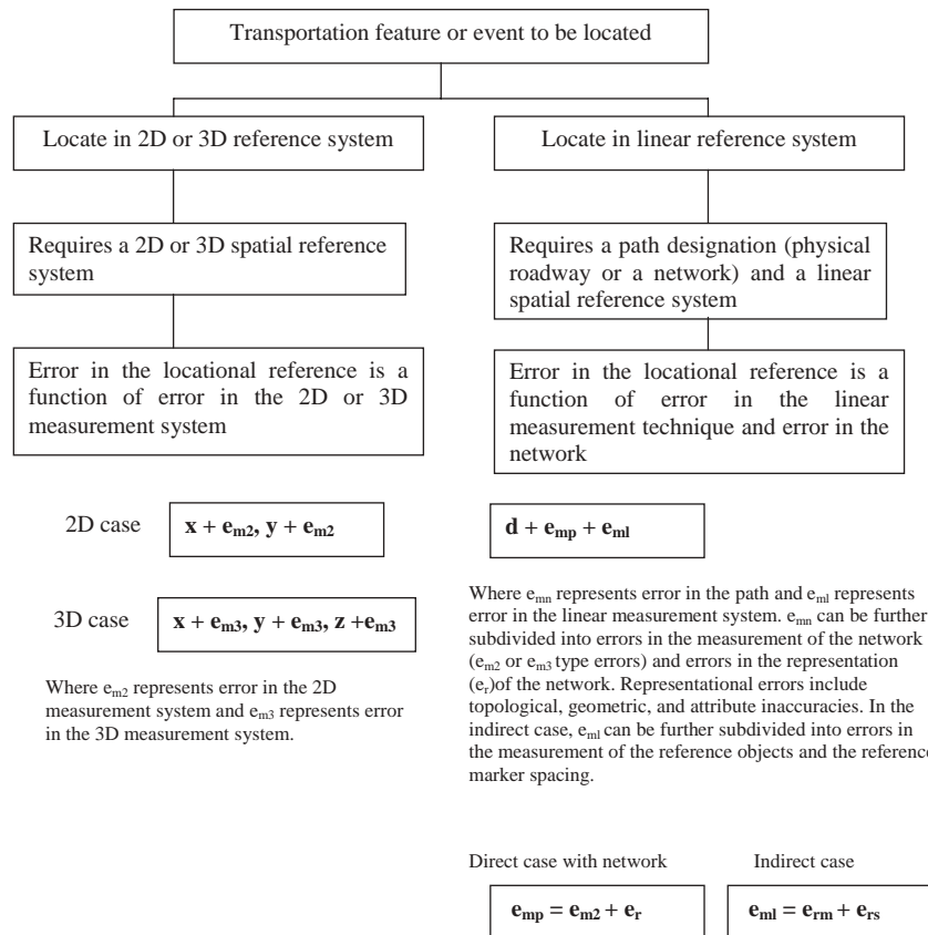
Figure 2-5. Outline of error sources associated with the process of assigning locational references to transportation features.
