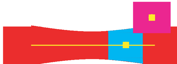
Figure 2-17. Combination of linear feature and 2D network.
