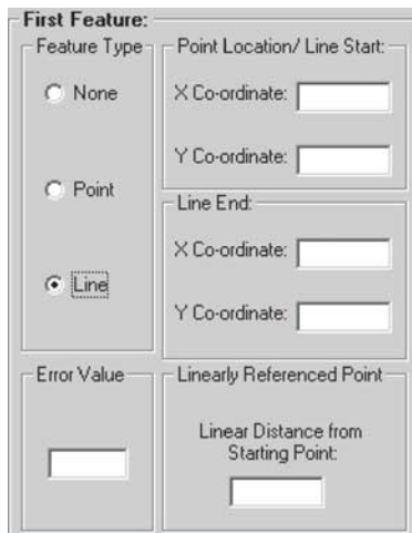
Figure A-3. Feature co-ordinates and associated error value.
