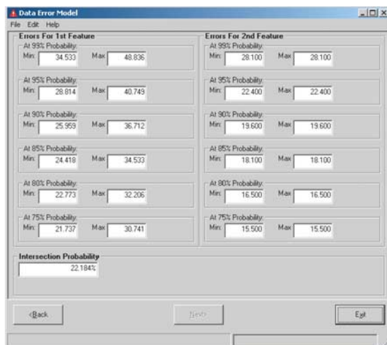
Figure A-5. Error analysis output window.
