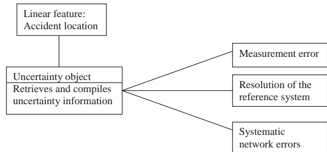
Figure 2-16. Detailed input requirements.
