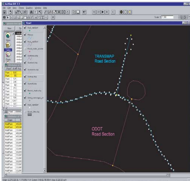
Figure 3-1. Example of intersection of two line features.
