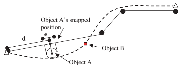
Figure 3-9. Transformation of nominal accuracy to distance error.
