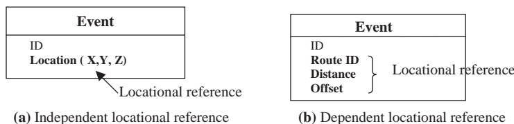
Figure 2-4. Distinction between locational references.
