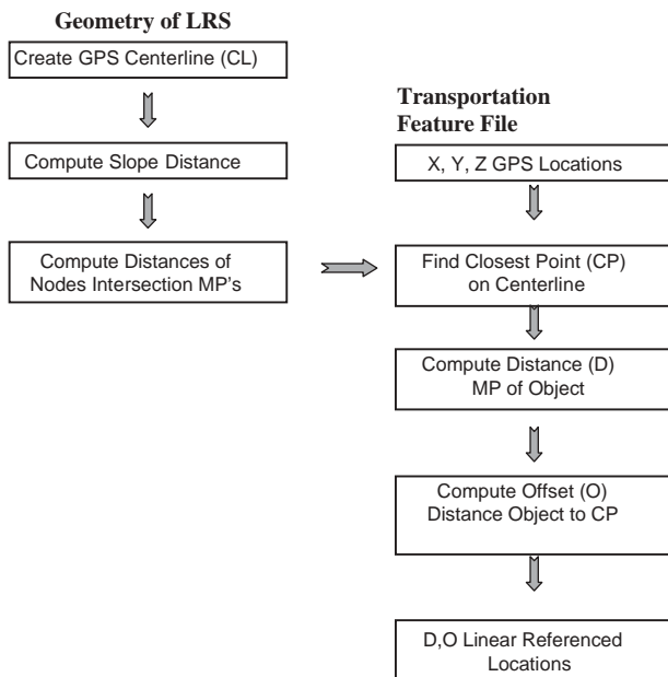
Figure 2-10. Steps in transformation of data for GPS to LRS.
