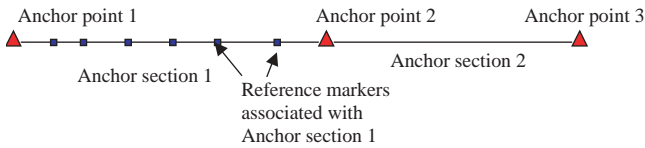
Figure 3-5. Components of linear datum.
