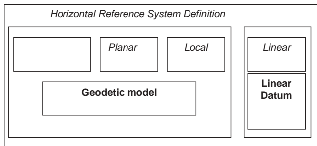
Figure 3-7. Recommended horizontal reference system.
