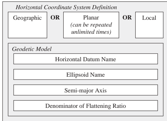
Figure 3-6. Current CSDGM horizontal coordinate system definition elements.
