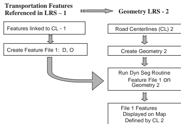
Figure 2-11. Steps in transformation of data from LRS-1 to LRS-2.
