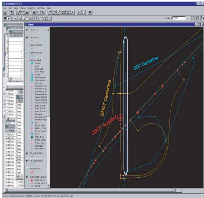
Figure 3-3. Comparison of two data sets with similar accuracy.
