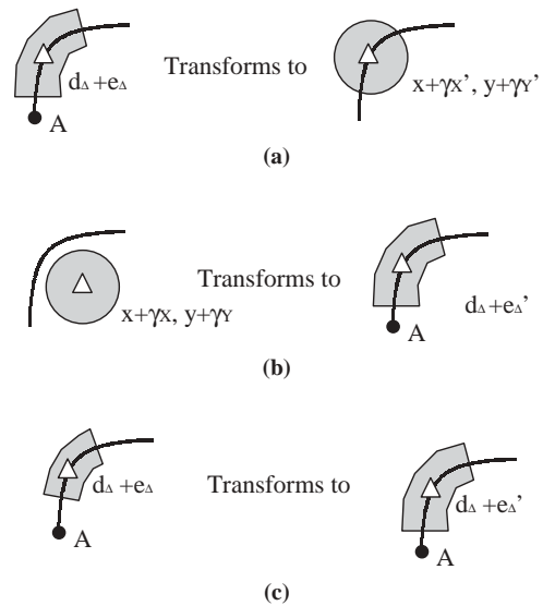
Figure 2-9. Examples of errors associated with the transformation types.
