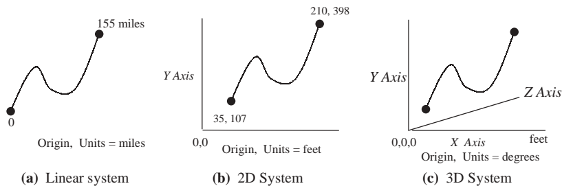
Figure 2-2. Components of spatial reference systems.
