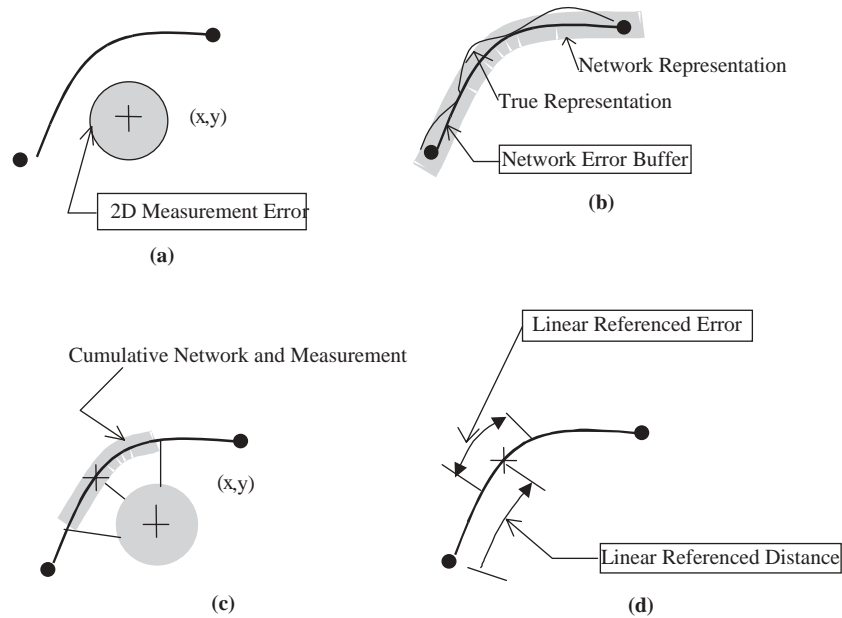
Figure 2-6. Schematic representation of positional data error.
