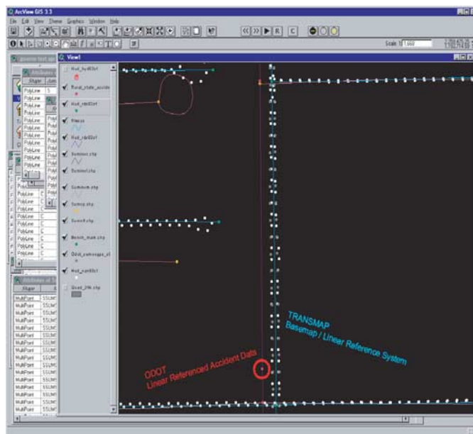
Figure 3-2. Example of intersection of a point and line features.
