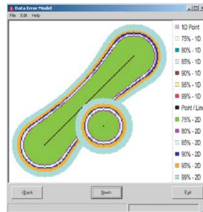
Figure A-4. The image window.
