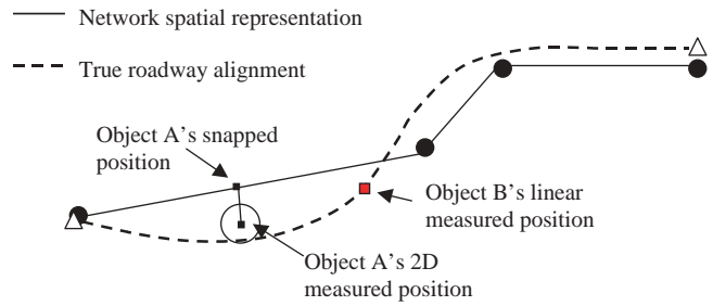
Figure 3-8. Transformation of 2D-measured position to LR position.
