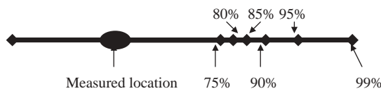
Figure 2-14. Probability zones of a one-dimensional point feature.
